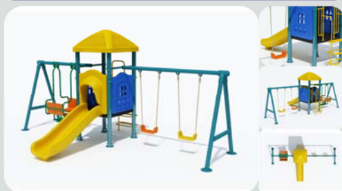
Size:650x380x330cm Safety Area:850x680cm
